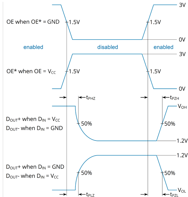
Figure 5. Driver High-Z Delay Waveforms
